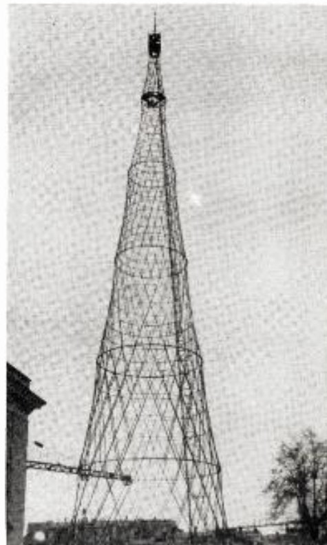
A Russian broadcasting tower, with its maze of cross-members, spirals skyward.
